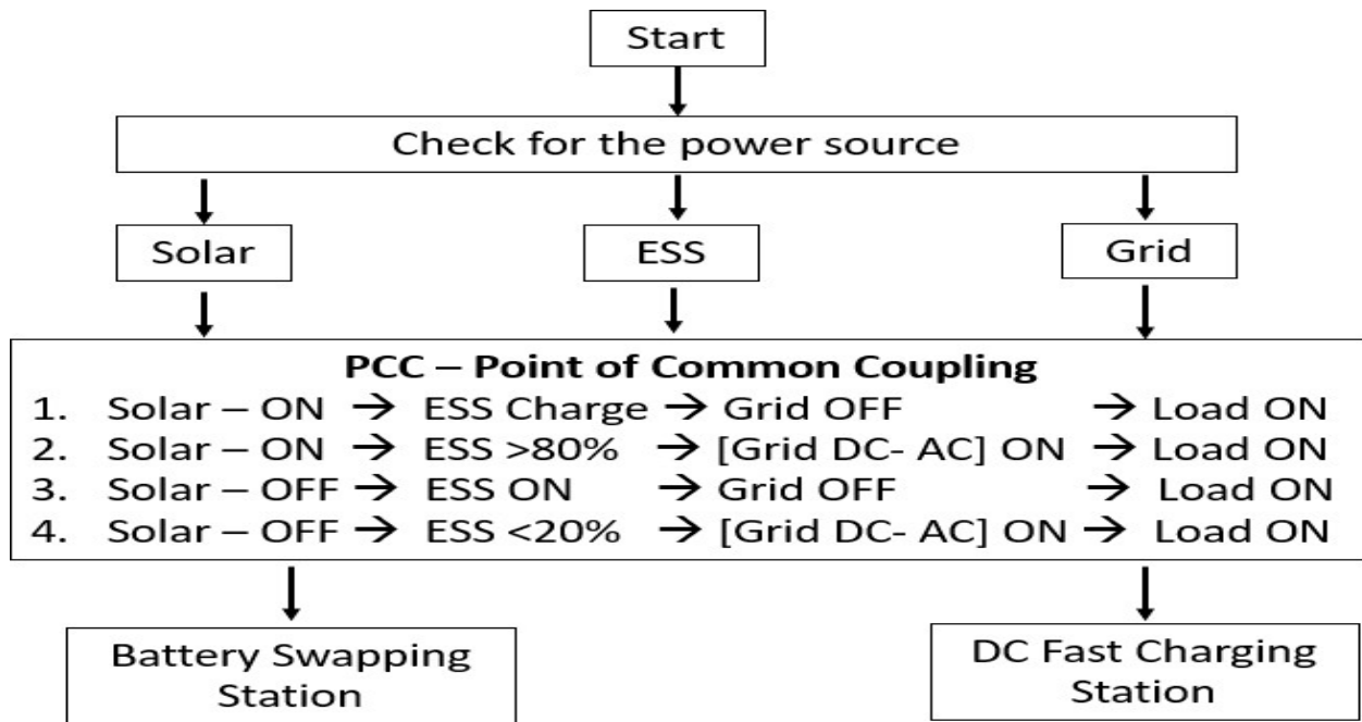
Fig 10 : PCC Control Flow
